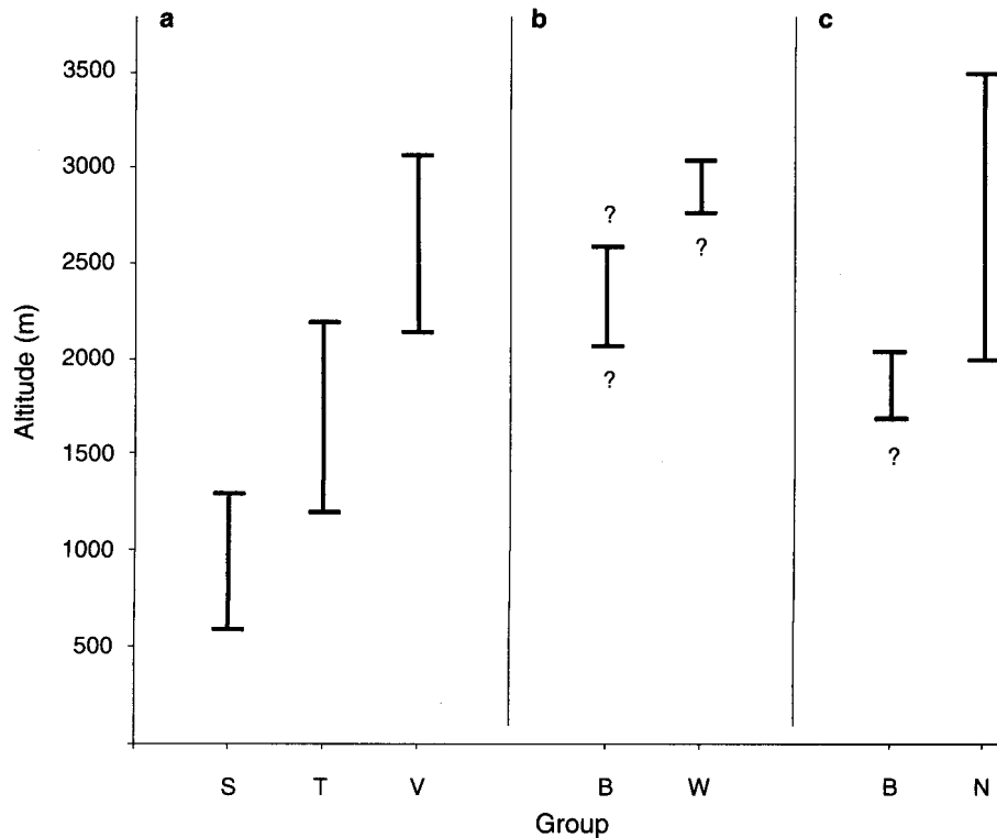
Figure 12. Altitudinal distributions (field and museums combined) in (a) Sichuan, Gansu and Shaanxi provinces, China (S, soror ; T, tephrocephalus ; V, valentini ); (b) Uttar Pradesh, India (B, burkii ; W, whistleri ); and (c) West Bengal (India), Sikkim and Bhutan (B, burkii ; N, nemorialis ). Lower limit of burkii is unknown, as is distribution of this and whistleri in the range 2600 to 2775 m in the western Himalayas.
