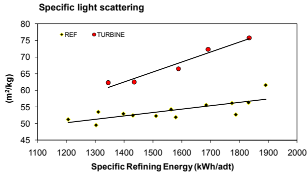
Fig 11. Specific light scattering increase with about 20% when using Turbine segments.
