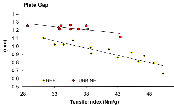
Fig 13. Compared to reference segments the plate gap increases at same tensile index when using Turbine segments.
