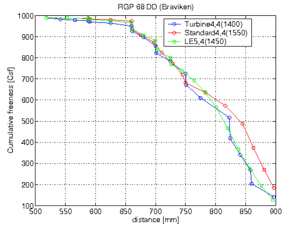
Fig 7. Cumulative CSF simulations for tested segment types.
