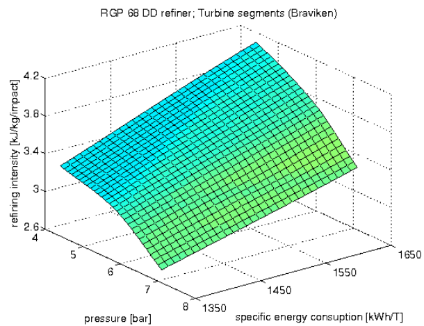
Fig 6. The intensity for the Turbine segment as a function of specific refining energy and pressure is different reference segments.
