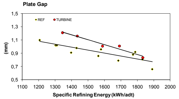
Fig 12. Plate gap was increased compared to similar tensile index when using Turbine segments.
