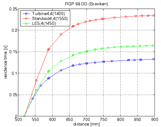
Fig 2. Illustration of calculated minimum fibre residence time. The Turbine segment minimum residence time is half of the reference, which shows that Turbine segments are more feeding.
