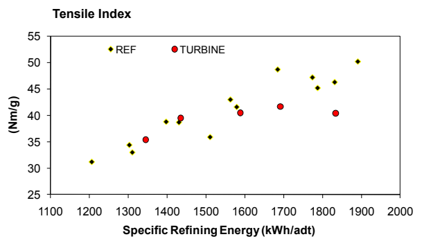
Fig 8. The tensile index development is similar for reference and Turbine segments. However, this tensile index development is constant for Turbine segments above 1600 kWh/adt.
