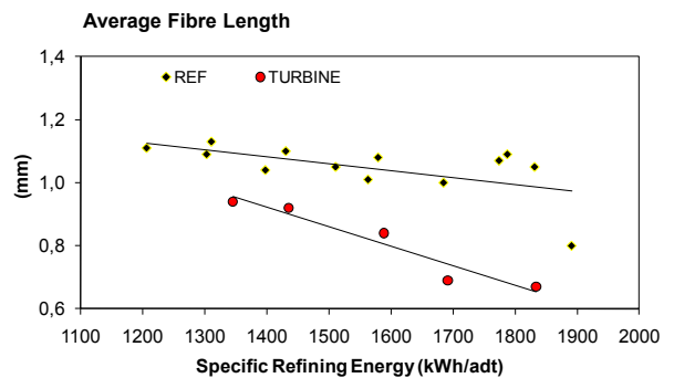
Fig 9. Turbine segments produce a pulp with shorter average fibre length compared to reference segments. The reduction is largest at high SEC.
