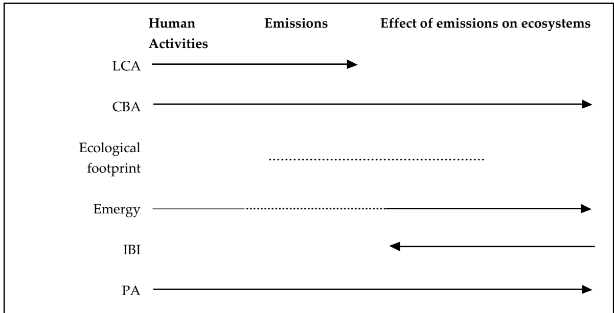
Figure 5. The different methods respond to human activities, emissions and effect of emissions on ecosystems.
