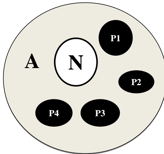
Figure 1 Anomaly detection
