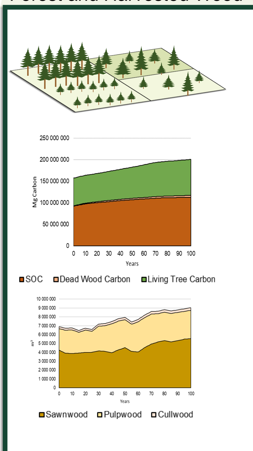
Biogenic Carbon Pools in Forest and Harvested Wood
