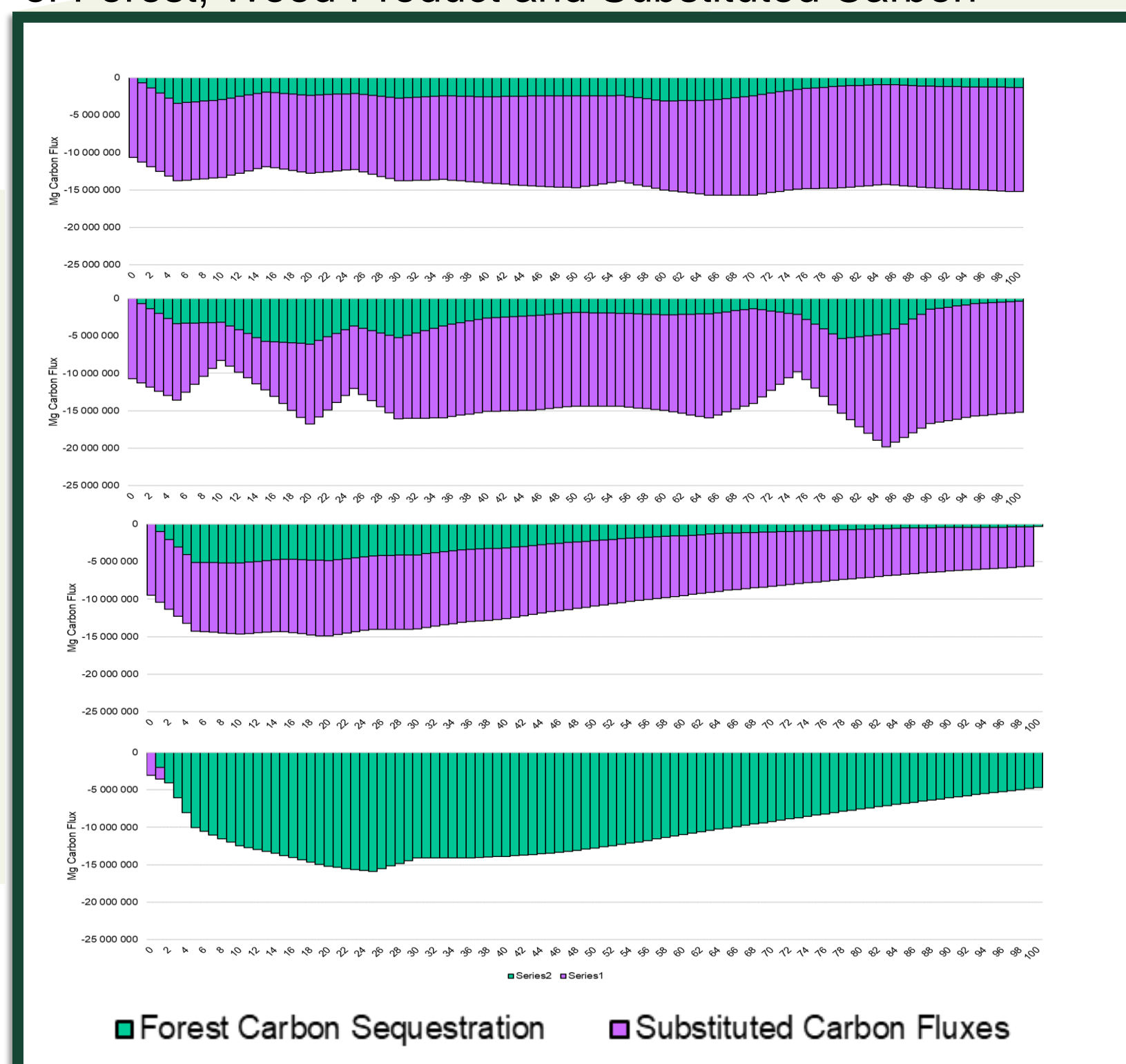
Time-Dynamic Carbon Model of Forest, Wood Product and Substituted Carbon
