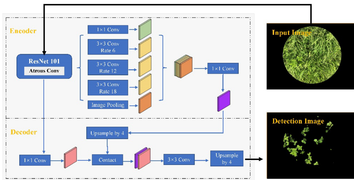
Fig. 5 Network structure of DeepLab V3+ model.
