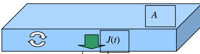
Figure 4. A constructed wetland modelled as being a well mixed body of water having constant volume and surface area.
