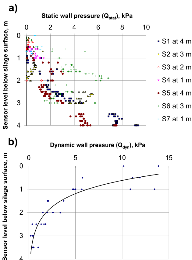
Fig. 4 – a) Example of static wall pressure load profile on a 4 m high bunker silo wall at first grass harvest with DM 27% and 591 recorded measurements from 7 sensors (S) placed at 1–4 m below the silo wall top. b) Example of dynamic wall pressure on the silo wall from the compaction machine (11.2–14.5 t) passing 0.1 m from the silo wall (4 m). The values show the load when the machine passes by the silo wall at different heights above the sensor positions.
