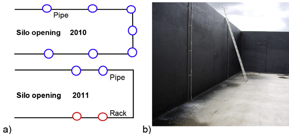
Fig. 3 – a) Placement in silo of 16 mm slotted measuring pipes for silage juice in 2010 where the distance between pipes was in proportion to silo length (approximate distance of 10 m apart) as seen from above. b) Measuring rack placed vertically along a silo wall, 6 m apart and 6 m from silo end in 2011.
