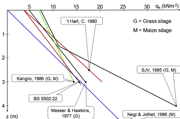
Fig. 1 – Current JBR guideline (SJV, 1995) compared with other guidelines and recommendations for silo wall load. The vertical axis ( z ) represents the distance below the silage top surface and the horizontal axis ( q_h ) the horizontal pressure on the silo wall given in different guidelines.
