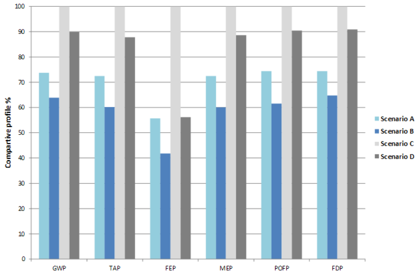
Figure 9. Comparative environmental impacts of the evaluated scenarios (study III). Acronyms: A, Swedish conventional supply chains; B, Swedish integrated supply chains; C, Canadian conventional supply chains; D, Canadian biomass dedicated supply chains.
